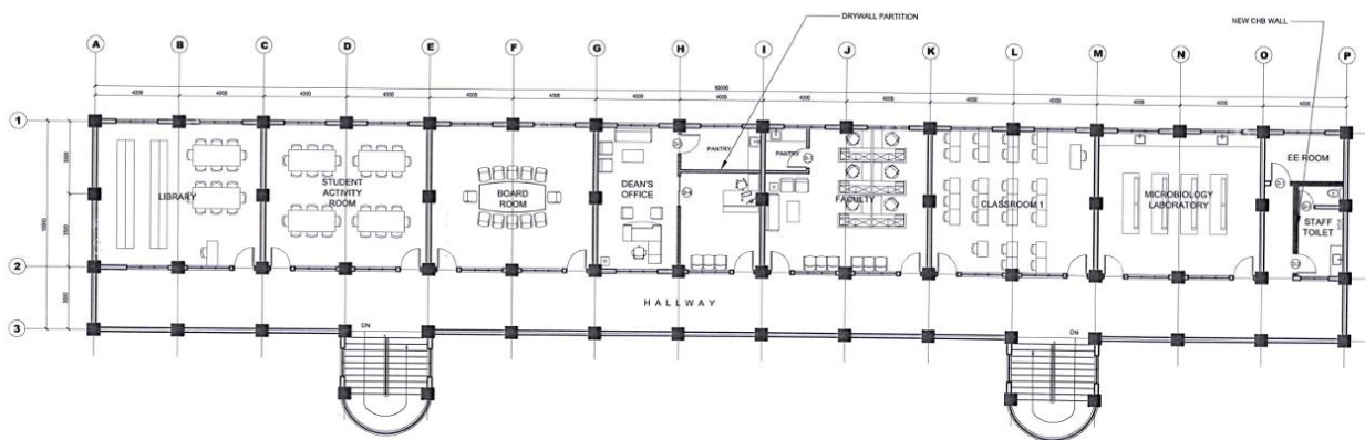
A-1 1/1 SCALE 1:175 MTS. PROPOSED THIRD FLOOR PLAN
