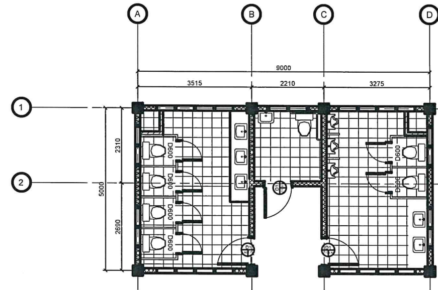
01 FLOOR PLAN LAYOUT AR1 SCALE 1:100 MTS.
