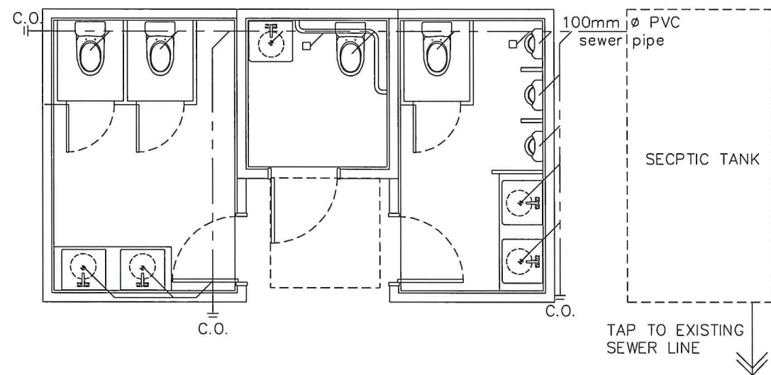
SANITARY LINE
