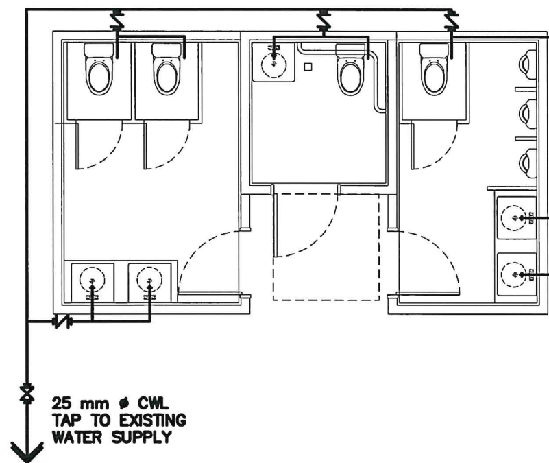
WATER LINE
