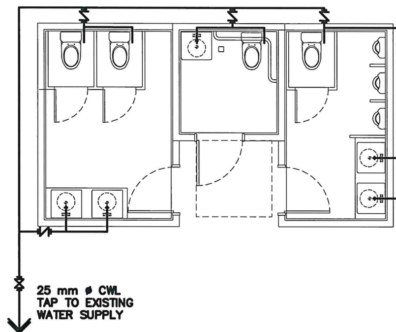
WATER LINE
