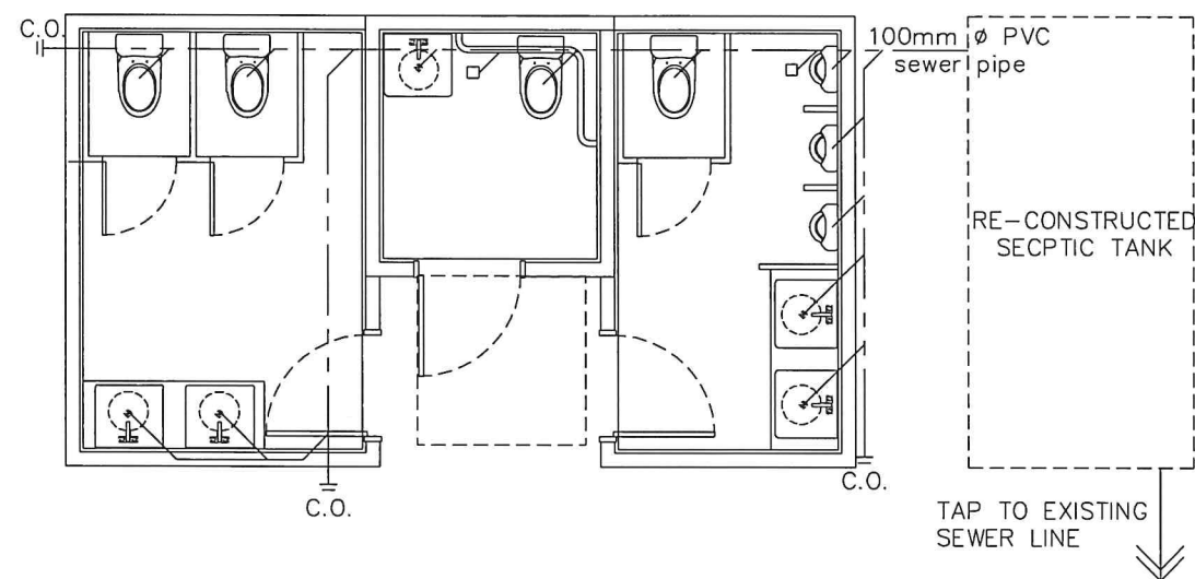
SANITARY LINE
